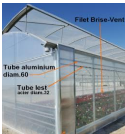
Roll-Up system
